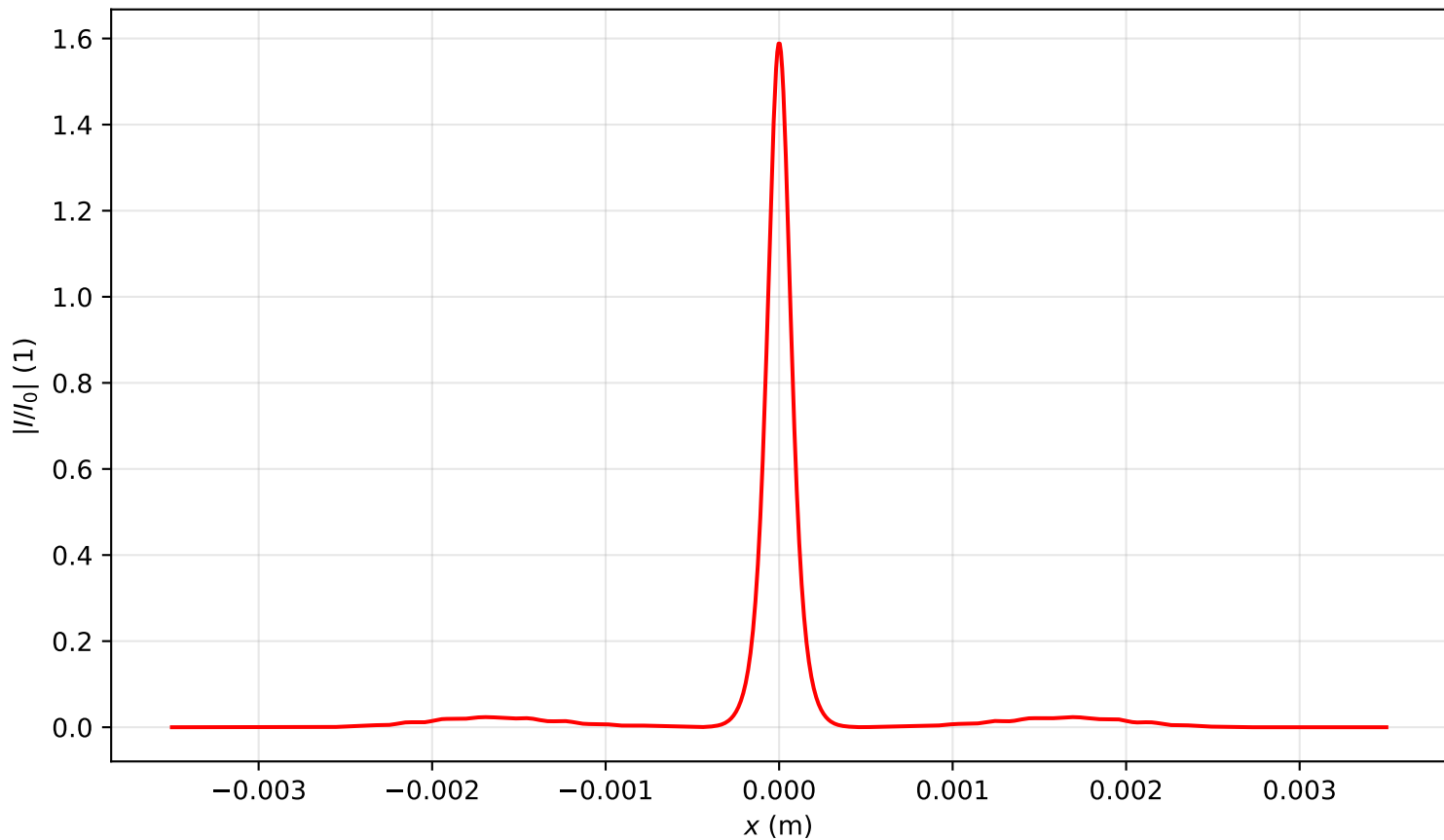
Intensity profile I(x, y = 0, z = 1.433)/I_0 , P_{in}=8.0P_{cr} , artificial time
